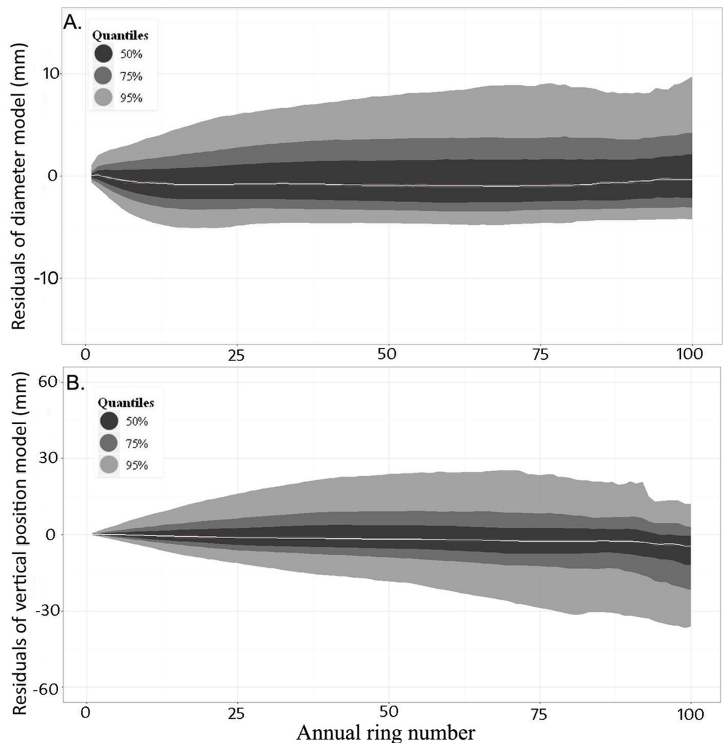
Figure 8 Distribution of the residuals (sorted by quantiles) against ring number when the model was applied to the evaluation dataset. (A) Knot diameter (Eq. (4) and Table 4) and (B) knot vertical position (Eq. (5) and Table 5). The grey line indicates the median of all observations for a given ring number. Contours provide the distribution around the median.
