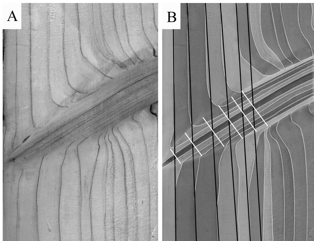
Figure 3 Inferring knot annual increments. (A) Example of ring width deformations around a knot; (B) extraction of the annual knot data.
