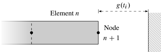
Figure 5. Rod approaching the rigid foundation at t_i
