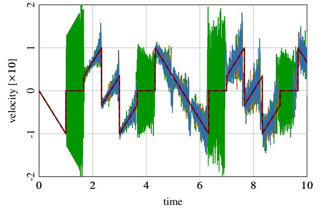
Figure 10. Contact node velocity for n = 100 : Exact Sol. [---], WFEM [—], FEM [—], Siconos ( e = 0 ) [—] and Siconos ( e = 1 ) [—]
