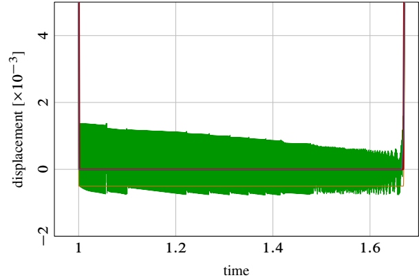
Figure 13. Gibbs' phenomenon for n = 500 : WFEM [—], FEM [—], Siconos ( e = 0 ) [—] and Siconos ( e = 1 ) [—]
