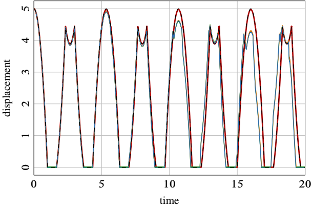
Figure 12. Contact node displacement for n = 500 : Exact sol. [- - -], WFEM [—], FEM [—], Siconos ( e = 0 ) [—] and Siconos ( e = 1 ) [—]
