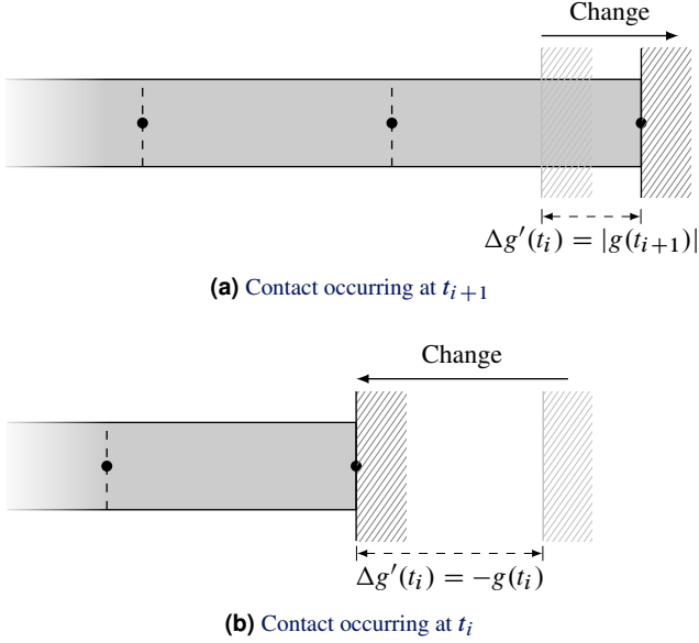
Figure 7. Temporary change to the position of the rigid foundation
