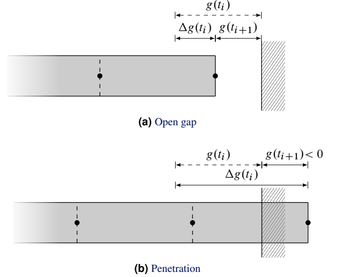
Figure 6. Possible contact configurations during time step \Delta t
