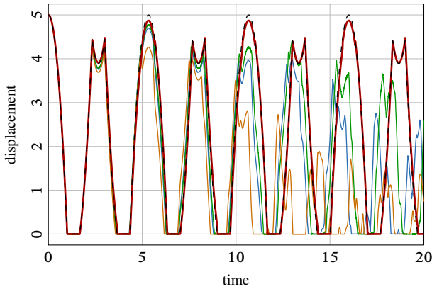
Figure 8. Contact node displacement for n = 100 : Exact Sol. [---], WFEM [—], FEM [—], Siconos ( e = 0 ) [—] and Siconos ( e = 1 ) [—]
