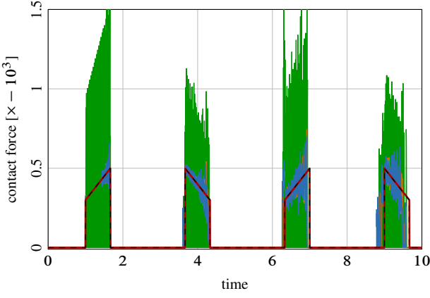
Figure 11. Contact force for n = 100 : Exact sol. [- - -], WFEM [—], FEM [—], Siconos ( e = 0 ) [—] and Siconos ( e = 1 ) [—]
