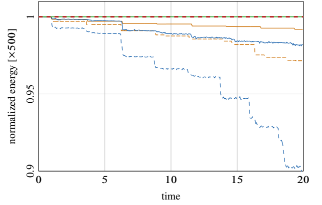
Figure 14. Normalized energy for n = 100 : FEM [- - -], Siconos ( e = 0 ) [- - -]; n = 500 : FEM [—], Siconos ( e = 0 ) [—]; Siconos ( e = 1 ) [—]; WFEM [- - -]
