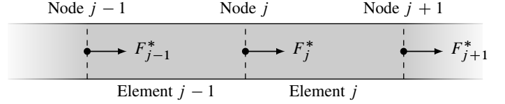
Figure 2. External equivalent nodal forces
