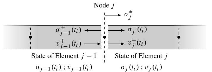
Figure 4. Interaction between elements j - 1 and j at time t_i
