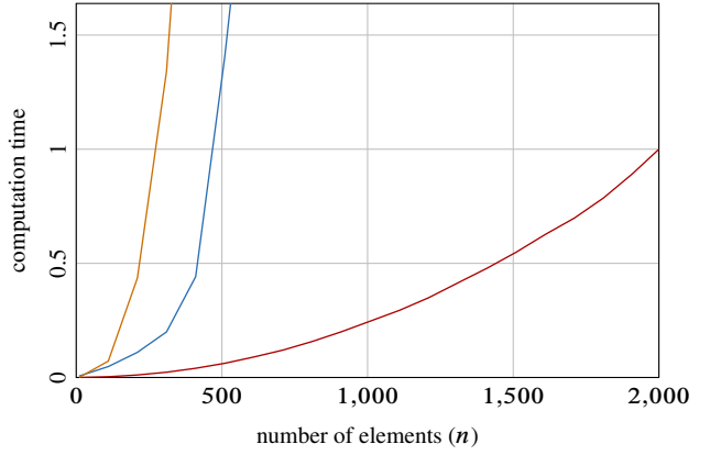
Figure 15. Computation time: WFEM [—], FEM [—] and Siconos ( e = 0, e = 1 ) [—]
