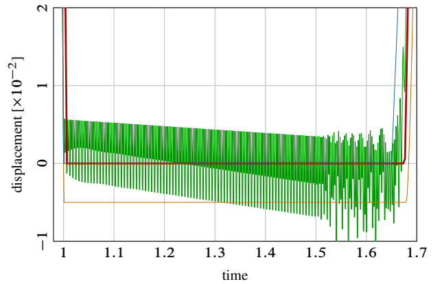
Figure 9. Gibb’s phenomenon for n = 100 : WFEM [—], FEM [—], Siconos ( e = 0 ) [—] and Siconos ( e = 1 ) [—]
