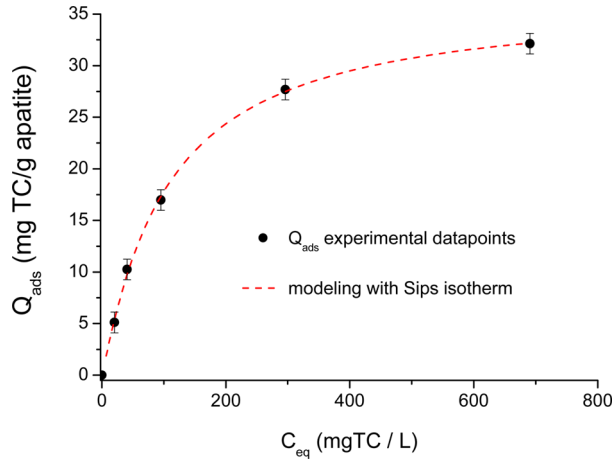
Figure 5. Adsorption isotherm (at 22 °C) of TC on biomimetic apatite matured 1 day and fit with the Sips isotherm model.
