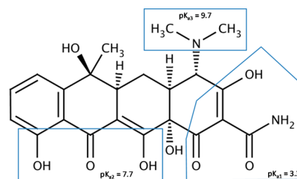
Figure 1. Chemical formula of tetracycline (TC).
