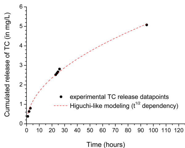
Figure 6. TC release from pelletized nanocrystalline apatite in recirculation cell (water, ambient temperature, neutral pH).
