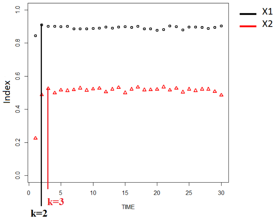
Figure 2: Plot of Sobol indices applied to model (48) in function of k .
