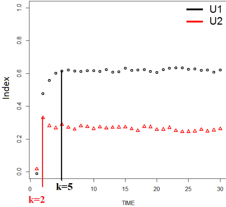
Figure 4: Plot of Sobol indices applied to model (56)
