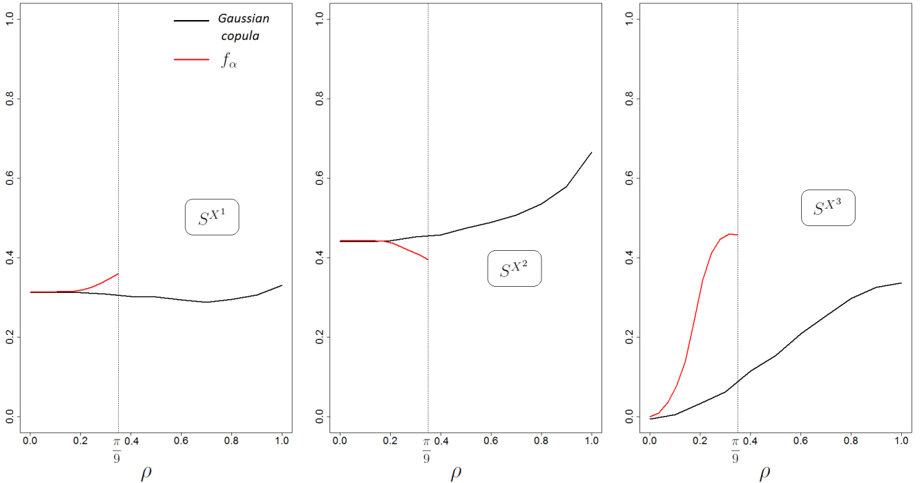
Figure 1: Sensitivity indices for different values of \rho' applied to the Ishigami model for the Gaussian copula and the f_\alpha copula
