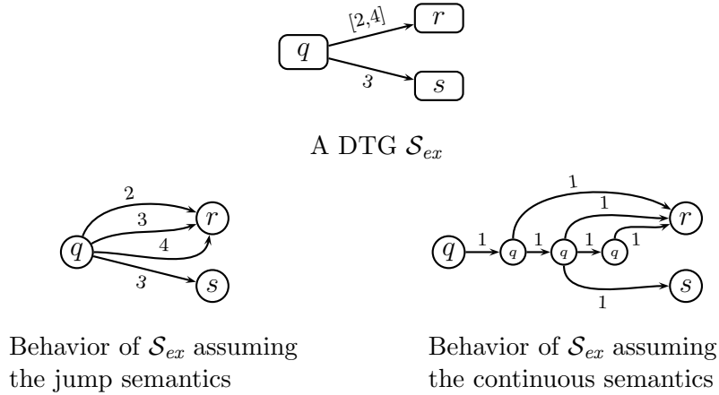
Fig. 2. Two different semantics for a DTG
