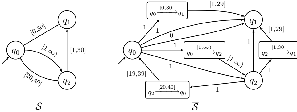
Fig. 6. Reduction from continuous early to continuous late semantics
