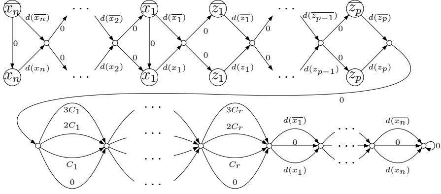
Fig. A.1. Kripke structure S_{\mathcal{I}} associated with SNSAT instance \mathcal{I}
