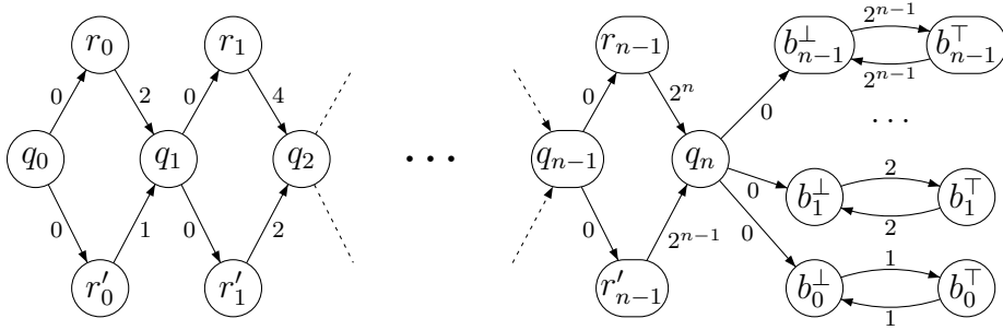
Fig. B.1. DTG \mathcal{S}_{\Phi} associated with QBF instance \Phi
