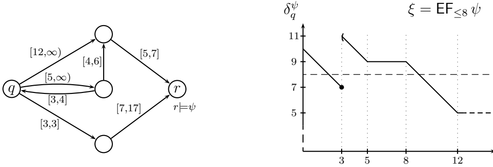
Fig. 4. An example of the duration function for a simple DKS
