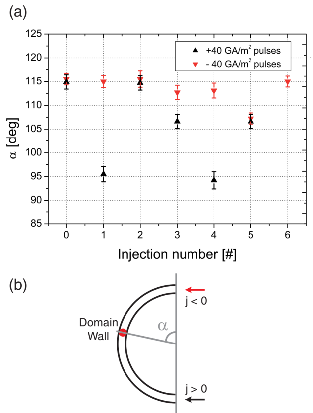
Figure 4. (a) Position of the domain wall center in a 2\ \mu\text{m} wide LSMO half-ring structure after a series of injections of pulses of 4 \times 10^{10}\ \text{A m}^{-2} . The black upward triangles and the red downward triangles refer to two different injection series. The half-ring structure was initialized by a magnetic field before each series of injections. The sign of the current density refers to the convention illustrated in (b), where the arrows indicate the direction of the current; (b) sketch of an LSMO half-structure, illustrating the angle convention ( \alpha ) and sign for the current density for the data points presented in (a). The single XMCD-PEEM images employed to generate the data in (a) are shown in the supplementary data ( stacks.iop.org/JPhysCM/26/456003/mmedia ).
