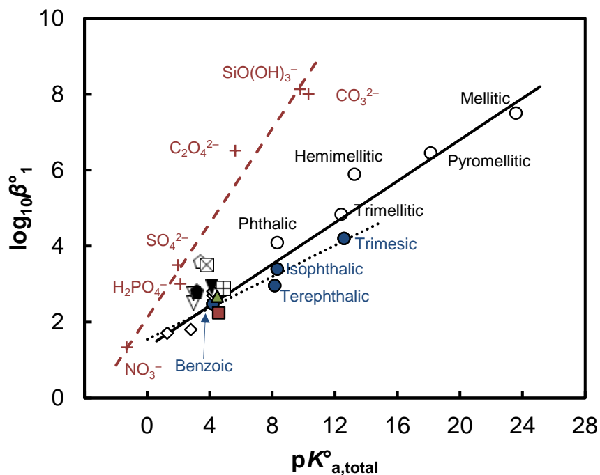
Figure 6. Linear free energy relationships between \log_{10}\beta^{\circ}_1 and pK_{a}^{\circ} for complexation of \text{AmSO}_4^+ , \text{AmCO}_3^+ , \text{AmH}_2\text{PO}_4^{2+} , \text{AmC}_2\text{O}_4^+ , \text{AmSiO}(\text{OH})_3^{2+} , and \text{AmNO}_3^{2+} (red cross from [59,81], dashed line is the linear correlation), experimental results from this study ( \text{EuProtoH}_2^{2+} green triangle, and \text{EuPhbH}^{2+} red square), data from aromatic (poly)carboxylic acids [24] (blue circles are non-chelate, open circles are possible chelates), \text{Eu}^{3+} complexes with acetic/chloroacetic (from SI), and phenylacetic acid (from [6,9] in Table 1, open diamonds); complex of \text{Eu}^{3+} with propionic acid [70] (straight-crossed square); complexes of \text{Am}^{3+} or \text{Eu}^{3+} with salicylic [5,7,36] (open inverted triangles), and \text{Eu}(\text{III}) with o-methoxybenzoic (closed inverted triangle), mandelic (2-hydroxy-2-phenylacetic acid, open pentagon), \alpha -methoxyphenylacetic (closed pentagon) acids [5], and lactic acid (tilted-crossed square) [77] are shown for comparison; the plain line is the correlation in ref. [24] between \log_{10}\beta^{\circ} and pK_{a}^{\circ} recalculated at 0 ionic strength using Davies equation [74]; the dotted line is the correlation accounting only for the non-chelate ligands (blue circles).
