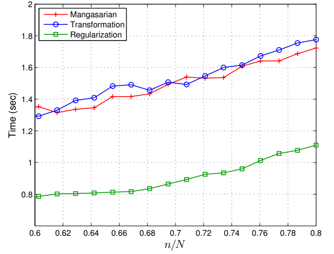
Figure 5. Computational time in seconds of Mangasarian and Recht's approach [8], regularization- and transform-based methods for the case p = 2 and N = 256 .
