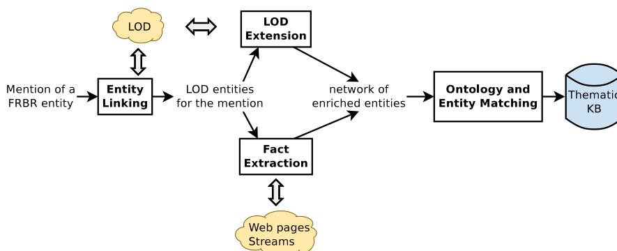
Fig. 1. Framework for building thematic knowledge bases
