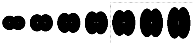
Fig. 3. Ultimate points (white) of elliptical fused objects (black).
