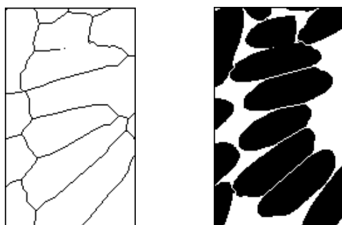
(a) - Gap-Filling. (b) - Result on binary image.
