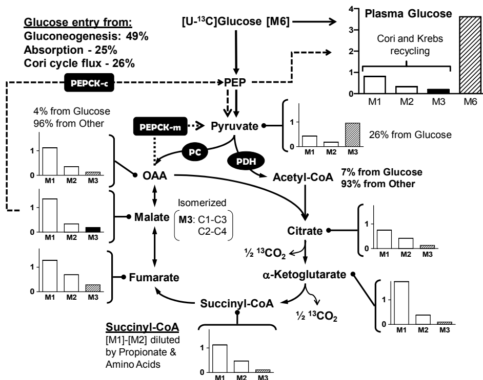
Figure 1. ^{13}\text{C} -Mass isotopomer distribution in plasma glucose and of hepatic Krebs cycle intermediates in a sheep given a constant infusion (32 h) of [\text{U-}^{13}\text{C}]_6 glucose into the duodenum (Bequette and El-Kadi, unpubl.). PC, pyruvate carboxylase; PDH, pyruvate dehydrogenase; PEPCK, phosphoenolpyruvate carboxykinase (c, cytosolic; m, mitochondrial).
