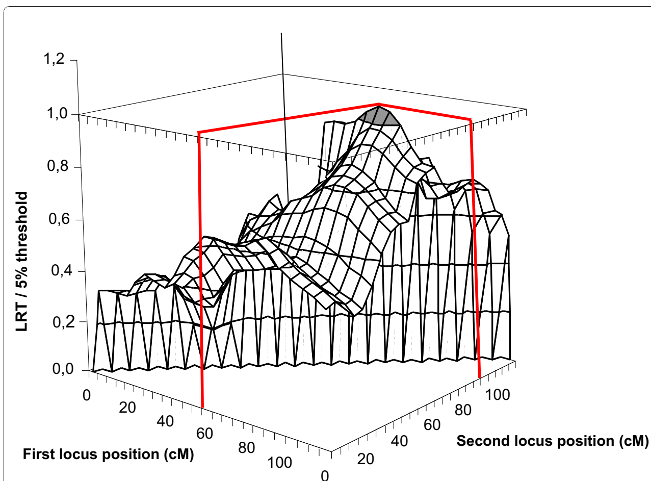
Figure 3 Two-QTL analysis results for Life Weight Gain on SSC4 with the combined pedigree. The z axis gives the value of the LRT divided by the 5% threshold at the chromosome-wide level, the surface shown in gray corresponding to a ratio higher than 1.
