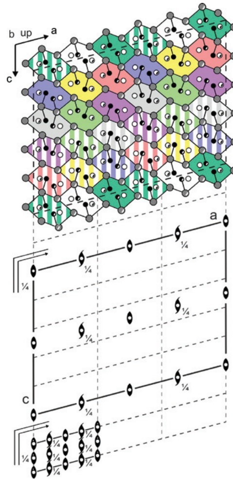
Fig. 12: Symmetry element thinning from the subcell at 300 K (bottom) to the 3a \times 5c approximant structure of CeCoAl at 90 K (middle and top). The black dashed lines symbolize the lattice of the subcell and the crescents mark the atoms with y = 1/2 . In the top part the 15 shortest Ce–Co distances are drawn and the coloration symbolizes the arrangement of these. Areas with same color but different pattern (filled and striped) are related by an inversion center.
