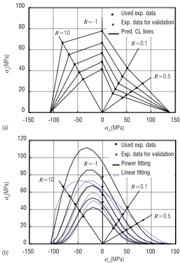
Figure 10 - Different types of CFLD: a - « multiple R-value CFL diagram »[50], b - power law [25]
