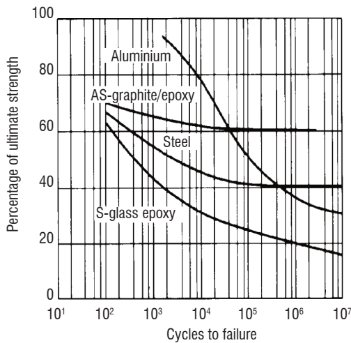
Figure 2 - Comparison of fatigue strengths of graphite/Epoxy, steel, fiber-glass/Epoxy and aluminum from Weeton et al. [91]
