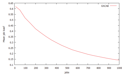
Figure 5: Job mean load with EACAB.
