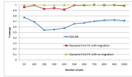
Figure 2: Energy of algorithms compared to dynamic first fit with unsorted hosts. Lower is better.
