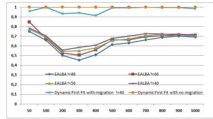
Figure 6: Variation of threshold vs energy gain with EACAB
