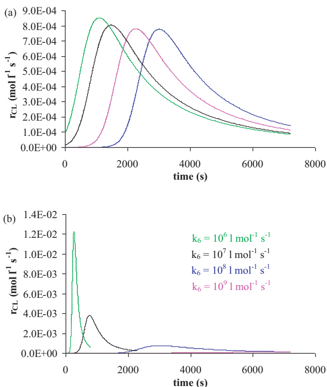
Fig. 3. Principle of adjustment of [\text{ROOH}]_0 (a) and k_6 (b). Other parameters were fixed equal to: [\text{R}^\bullet]=[\text{ROO}^\bullet]=0 , [\text{RH}]=6 \text{ mol L}^{-1} , k_{1b}=1 \times 10^{-2} \text{ L mol}^{-1} \text{ s}^{-1} , k_2=10^7 \text{ L mol}^{-1} \text{ s}^{-1} and k_3=100 \text{ L mol}^{-1} \text{ s}^{-1} , k_6=10^9 \text{ L mol}^{-1} \text{ s}^{-1} (a) and [\text{ROOH}]_0=10^{-2} \text{ mol L}^{-1} (b).
