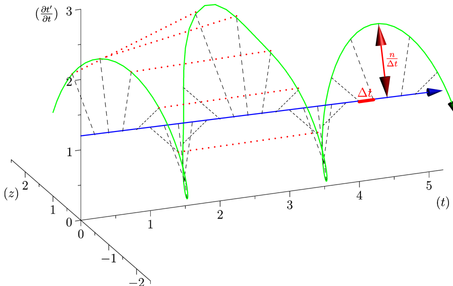
Figure 4: Renormalization and principles of variability representation. Here, we consider \frac{\partial \vec{\mathfrak{z}}_{\tau_i}(t, \theta)}{\partial t} and we renormalize the compactified time by n = 10 . A change of speed for the iteration m of the original compactified time appears as a sharp contrast between this iteration and its neighbors: iteration m - 1 , m + 1 , m - 10 , m + 10 . As a result, if there is a coherence for 10 successive iterations, we obtain a fully circular outgrowth or contraction (for an acceleration or a slowdown respectively).
