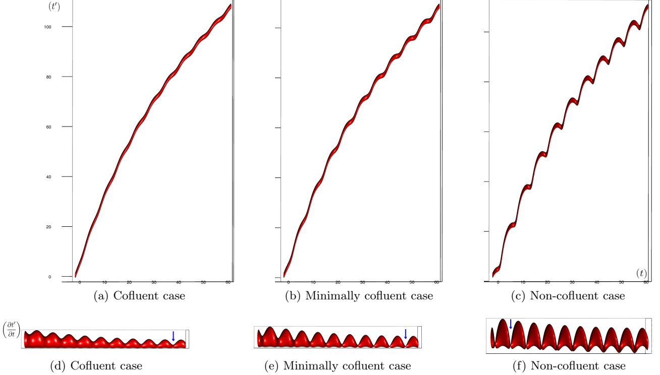
Figure 3: Illustration of the three scenari. TOP: the scheme \vec{\mathfrak{S}}_{\tau_i}(t, \theta) and BOTTOM its time derivative \frac{\partial \vec{\mathfrak{S}}_{\tau_i}(t, \theta)}{\partial t} . FROM LEFT TO RIGHT: Cofluent case, minimally cofluent case and non-cofluent case. Since the radius of the compacified time is proportional to its physical rate when looking at \frac{\partial \vec{\mathfrak{S}}_{\tau_i}(t, \theta)}{\partial t} (see §4.4.1), the bottom pictures allows to see when the slowest rate occurs (i.e.: when the radius is the smallest, blue arrow. Here respectively: for adults in figure 3d and 3e and for infants in 3f).
