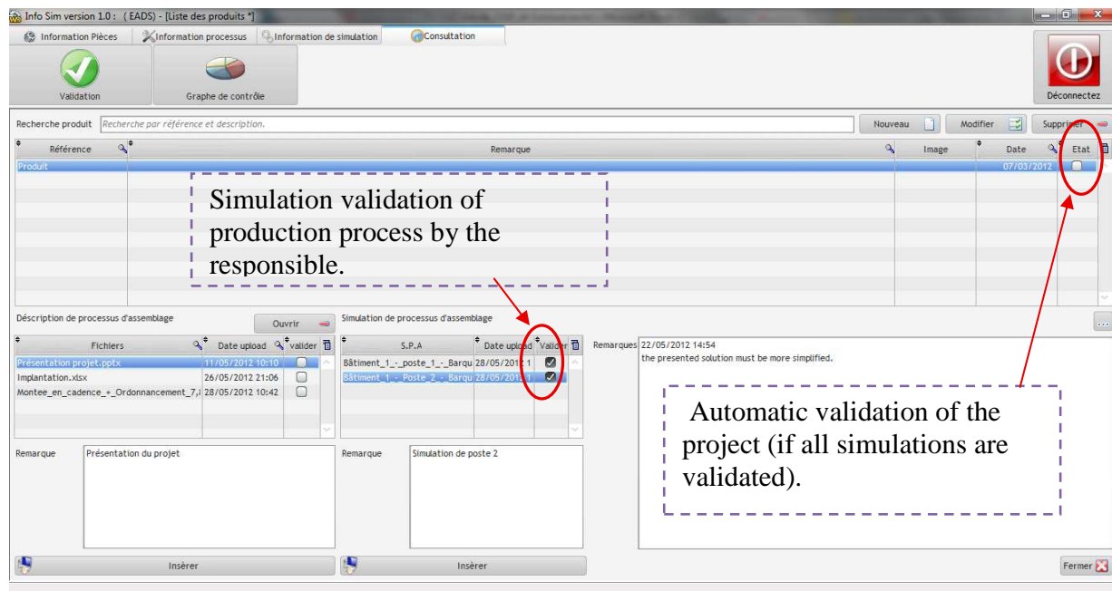
Figure 5. Simulation validation in the information system Info SIM
