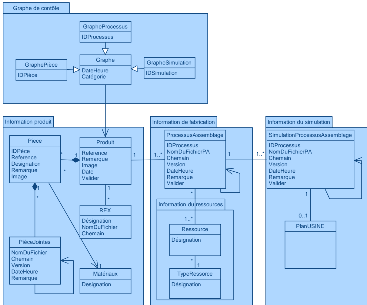
Figure 3. Logical Model of Info SIM
