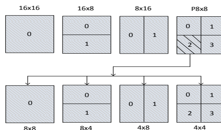
Fig. 6. Inter prediction modes
