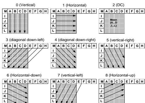
Fig. 2. Intra4x4 prediction modes
