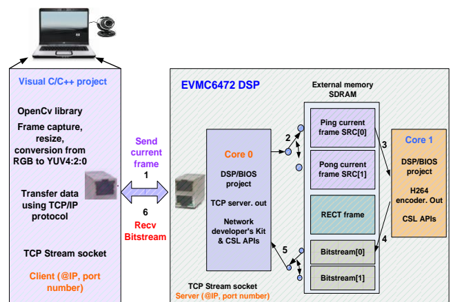
Fig. 17. Real time video encoding demo
