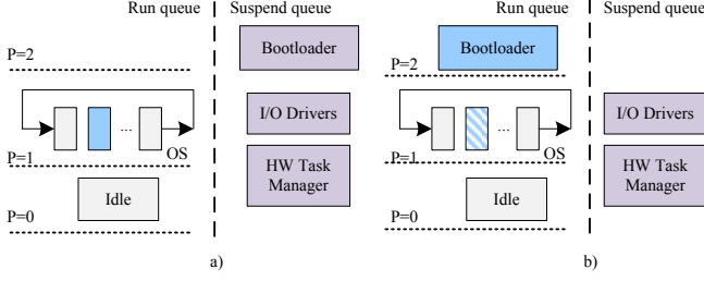
Figure 3. Scheduling Process. a) Guest OSes round-robin sharing CPU. b) User service bootloader is added to the run queue and preempts lower-priority VMs
