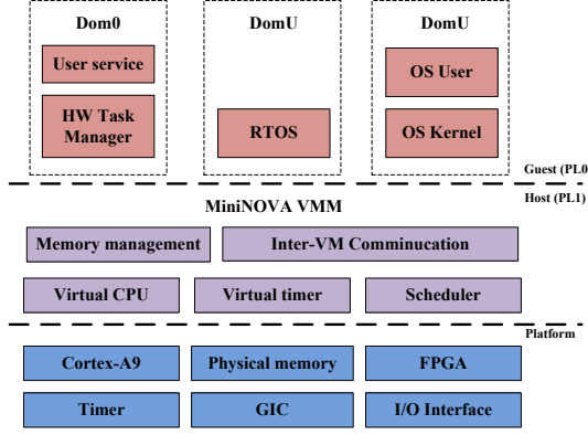
Figure 1. Mini-NOVA Architecture Overview
