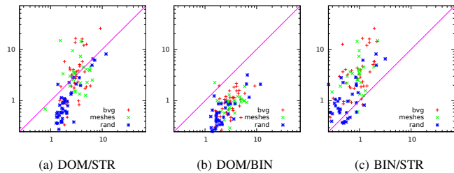
Figure 6. Speedups with 30 subproblems per worker: Each point (x, y) in (a) (resp. (b) and (c)) corresponds to an instance such that x is the speedup for DOM (resp. DOM and BIN) and y for STR (resp. BIN and STR).
