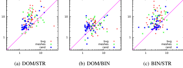
Figure 4. Speedup bounds without t_{dec} : Each point (x, y) in (a) (resp. (b) and (c)) corresponds to an instance such that x = t_0/t_{max} for DOM (resp. DOM and BIN) and y = t_0/t_{max} for STR (resp. BIN and STR).
