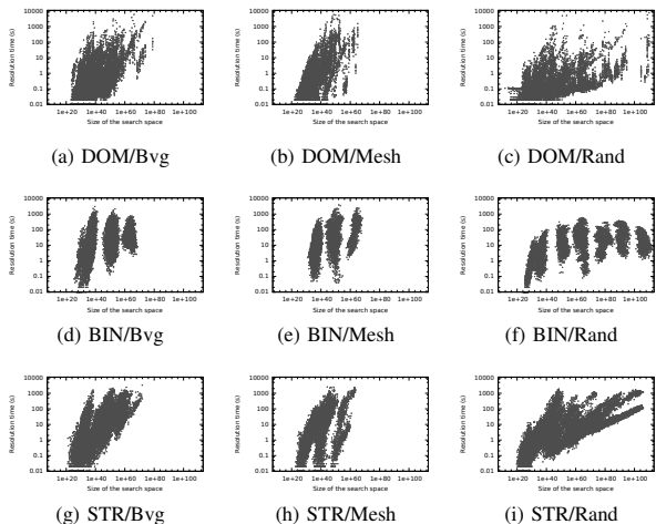
Figure 5. Size w.r.t. time: for each decomposition method d \in \{\text{DOM, BIN, STR}\} , and each instance class c \in \{\text{bvg, mesh, rand}\} , the subfigure d/c plots a point (x, y) for each subproblem obtained when decomposing an instance of c with d , where x is the size of the search space of this subproblem, and y is the time needed to solve it.
