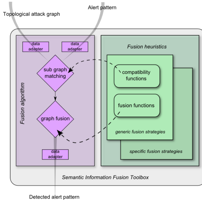
Fig. 3. Fusion architecture
