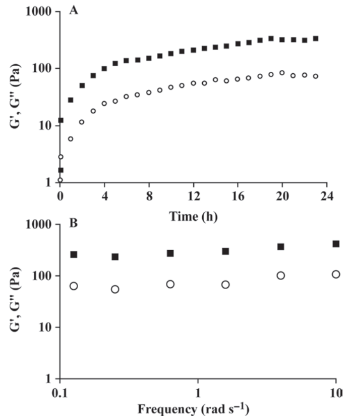
Figure 2. (A) Storage modulus ( G' ; ■) and loss modulus ( G'' ; ○) for acid milk gels acidified by glucono- \delta -lactone (GDL) under N_2H_2 conditions. (B) Mechanical spectrum of G' (■) and G'' (○) for acid milk gels acidified by GDL under N_2H_2 conditions.
