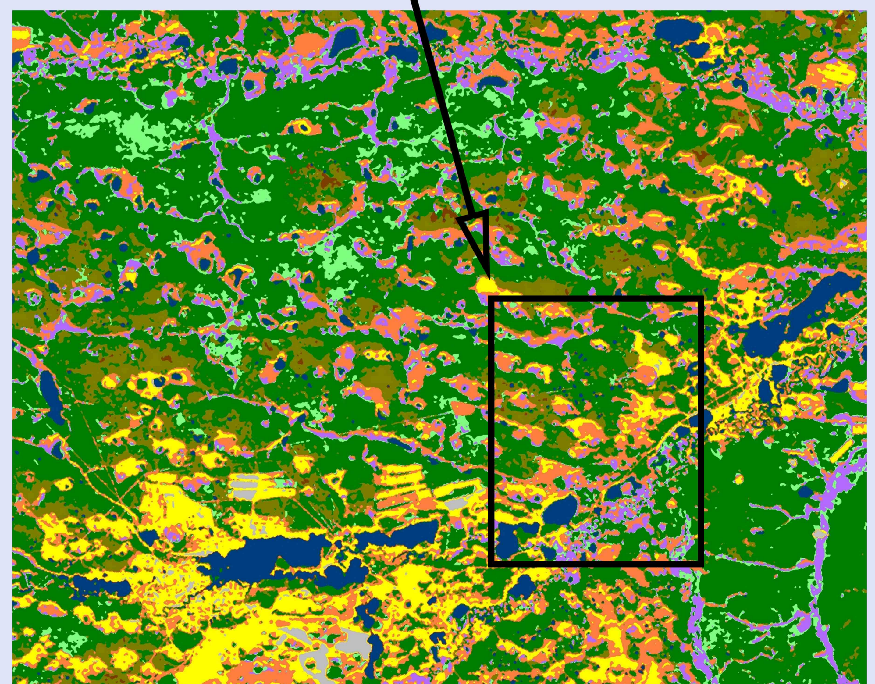
Landsat-ETM 2001 classification
