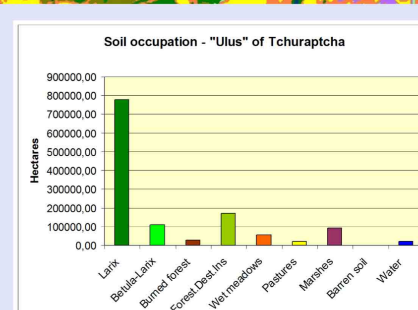
Landsat-ETM 2001 classification
