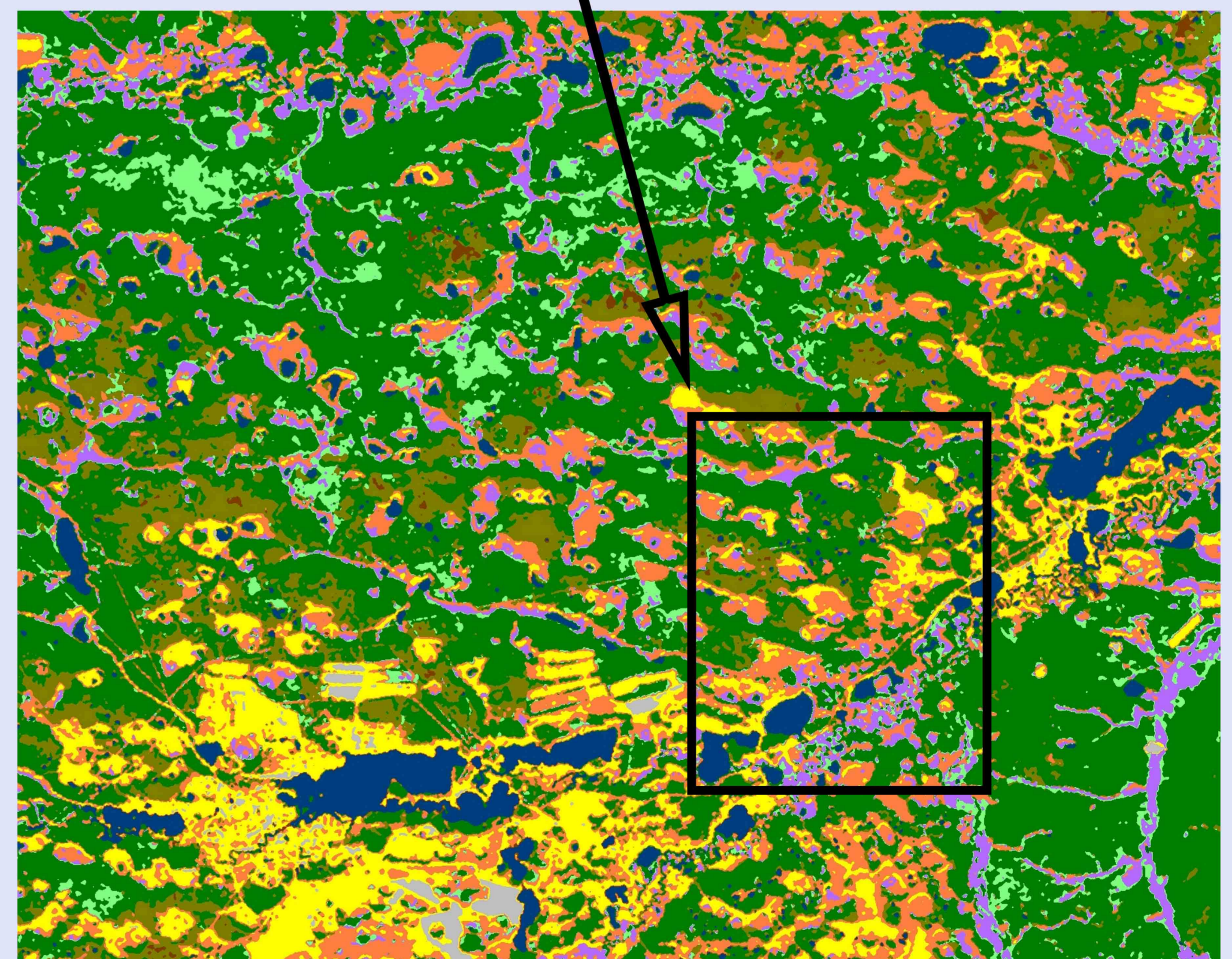
Landsat-ETM 2001 classification
