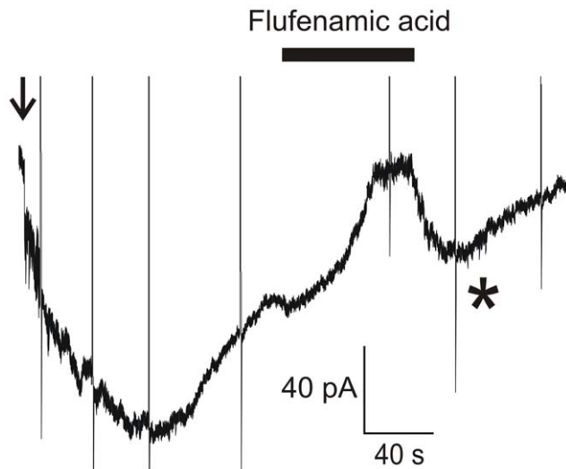
Figure 7. Cl - channel inhibitors reversibly block the SlitBest1b current. A) Application of 100 \mu M flufenamic acid on the steady state of the whole-cell Ca 2+ -activated current recorded at a holding potential of -60 mV. Recordings were done in low-Cl - external solution. Currents recorded during voltage protocols are truncated. The star indicates the transient current rebound observed after washing out flufenamic acid. The arrow indicates the transition from cell-attached to whole-cell configuration. doi:10.1371/journal.pone.0052691.g007
