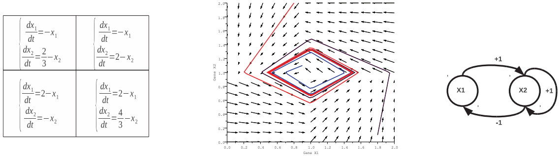
Figure 2: An example of biological cycle: the choice of the parameters here is \gamma_1 = \gamma_2 = \theta_1^1 = \theta_1^2 = \theta_2^1 = \theta_2^2 = 1 , k_1^0 = -k_1^2 = 2 , k_2^1 = \frac{4}{3} and k_2^2 = \frac{2}{3} . There are 4 boxes in which the system is linear. Whatever its initial condition, all trajectories will spiral toward a unique limit cycle.
