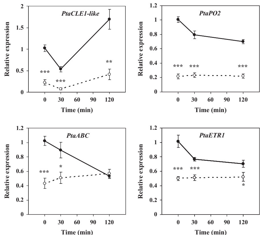
Fig. 4 Expression levels of four genes down-regulated in PtaZFP2 -overexpressing ( PtaZFP2 -OE) poplars (#39) without or after a transient stem bending. PtaZFP2 expression was monitored by real-time PCR (qPCR). Plants ( Populus tremula × Populus alba ) were treated with 17 \beta -estradiol (10 \mu M) for 4 d. The bent zone of stems was collected 30 and 120 min after a single transient bending. In each line and condition, the relative transcript abundance was determined by comparison with the gene expression level in 17 \beta -estradiol-treated wild-type (WT) plants using EF-1 \alpha transcript abundance as a reference. Closed circles, WT; open circles, #39. Represented values are means of five to seven biological replicates \pm SE. Asterisks indicate statistically significant differences (Student's t -test) between WT and PtaZFP2 -OE poplars: *, P < 0.05 ; **, P < 0.01 ; ***, P < 0.001 .
