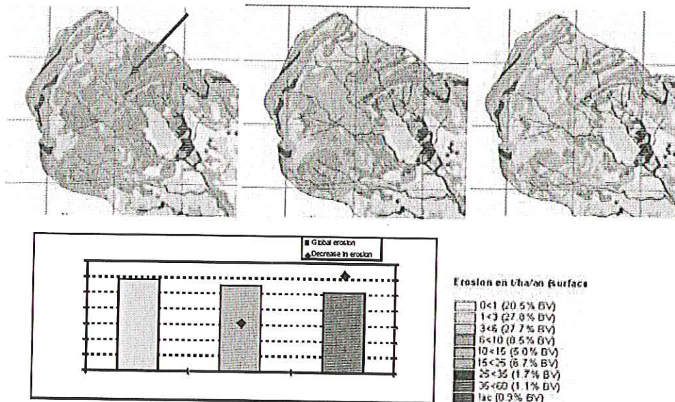
Figure 46. The Abdessadok Basin (partial), limiting erosion with the replacement of scrubland (left) on upstream lithosols by a young forest (center) becoming a mature adult (right).
