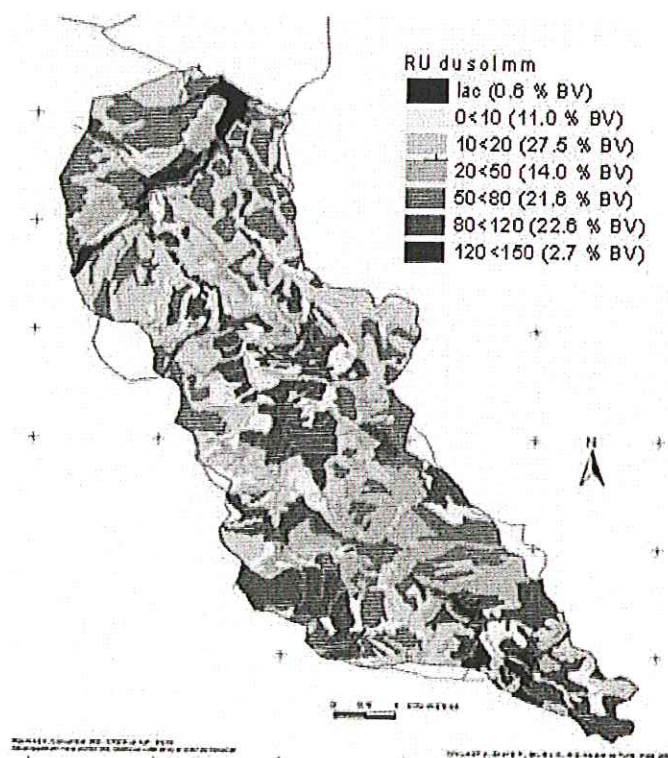
Figure 45. Map of isolines of soil usable water reserves UR. Source: Collinet et al. 2001.
