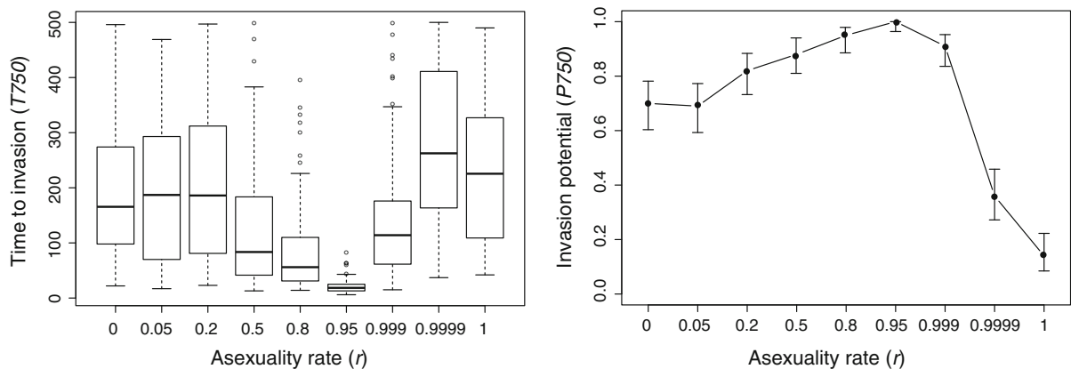
Fig. 3 Effect of asexuality rate ( r ) on the time to invasion ( T750 ) and invasion potential ( P750 , i.e. the proportion of successful invasions). Parameter values: \sigma_e^2 = 0 , \mu = 0.001 , \alpha^2 = 0.05 , D = 2.8 , m = 0.01
