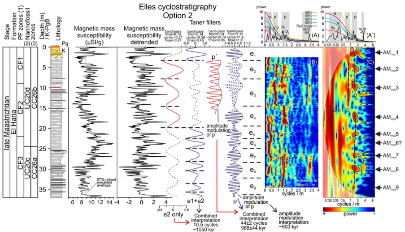
Fig. 4 : Cyclostratigraphic analysis of the Elles section (option 2). a 4\pi MTM with red noise model and \chi^2 significance levels. a' Same with a log2 scale on the x-axis. b Amplitude spectrogram of the time series. c Wavelet spectrum of the time series. sub-M sub-Milankovitch cyclicities
