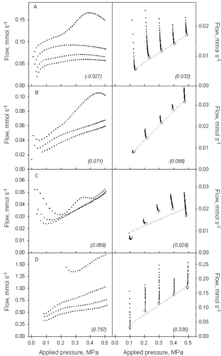
Figure 2. Typical time courses of water flow versus applied pressure during the measurement of root system hydraulic conductance with the HPFM using the transient mode (left column) and the dynamic mode (right column). Flow and pressure were recorded every 3 s, each point corresponds to one record. For the transient mode, pressure was increased at a rate of 5–8 kPa s -1 and k_r was estimated from the slope of the last 8 points. For dynamic mode, pressure was increased to the next step after 3 min at a given level, once the water flow was quasi-stable and k_r was calculated from the slope of the regression of the 5 points corresponding to the last recording of each step (open circle) if r^2 was higher than 0.95. For each plot, k_r is given between brackets (mmol s -1 MPa -1 ).
