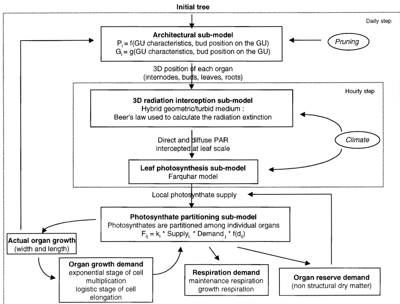
Figure 1. Schematic organisation of the model. ( P_i : budburst probability, G_i : growth potential, F_{ij} : photosynthate flux between a source i and a sink j , k_i : coefficient of matter conservation, f(d_{ij}) : function modulating the effect of the distance ( d_{ij} ) between a source i and a sink j ).
