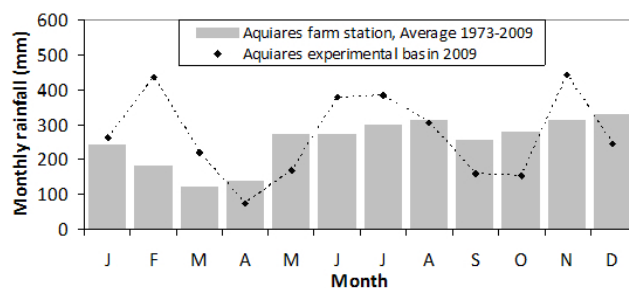
Fig. 2. Mean monthly rainfall at Aquiras farm station (period 1973–2009) compared to the rainfall in the experimental basin in 2009.
