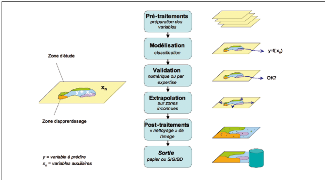
Figure 8 - Processing flowchart to supervised model.
