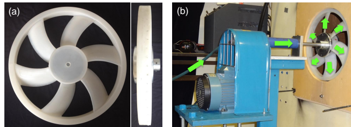
Figure 1: The hollow fan (a) and the fan drive system (b)
