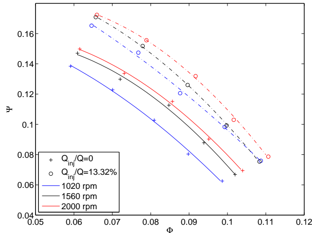
Figure 2: Comparison of aerodynamic characteristic of the axial fan for the case with and without internal flow and for 3 rotation speeds: 1020, 1560 and 2000 rpm
