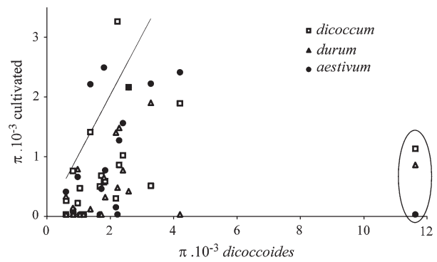
FIG. 5.—Joint patterns of nucleotide diversity observed in wild diccooides and cultivated relatives at 21 gene fragments, with each gene plotted 3 times. The \pi_{wild}/\pi_{cultivated} ranged from 0 to more than 1, depending on the gene considered. The line (slope = 1) indicates equivalent levels of diversity in diccooides and the cultivated taxa. The encircled points represent diversity at the HgA locus in the 3 cultivated groups.
