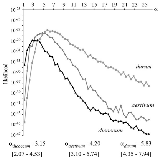
FIG. 4.—Likelihood (yaxis, logarithmic scale) profiles as a function of bottleneck intensity, \alpha (xaxis) for each cultivated group, based on the 21 loci ( \alpha = Ne_{diccooides}/Ne_{cultivated} ).
