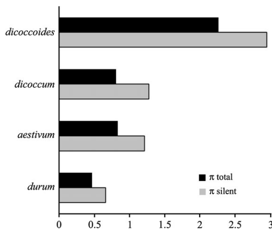
FIG. 3.—Nucleotide diversity ( \pi ) expressed in 10^{-3} in the wild ( dicoccoides ) and cultivated groups ( dicoccum , durum , and aestivum ). Total nucleotide diversity \pi_{total} was estimated for the whole sequence, whereas \pi_{silent} corresponds to nucleotide diversity for noncoding and synonymous sites only.
