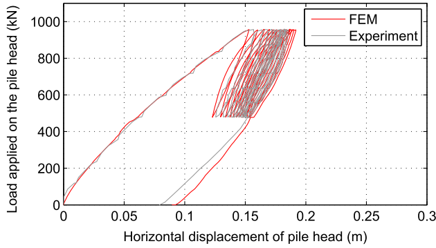
Fig. 6 FEM model with the von Wolffersdorff hypoplastic law and Rosquoët’s cyclic tests on a lateral loaded pile [64]
