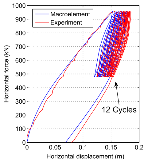
Fig. 9 Comparison between experimental results and macroelement response for cyclic horizontal loading test. Data from Rosquoët [64]
