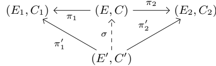
Fig. 9. Universal property of the product
