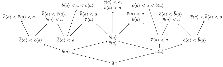
Fig. 3. (\bar{b}(a) \mid \bar{c}(a) \mid a) \setminus a in rigid families
