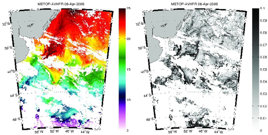
(a) METOP-AVHRR
