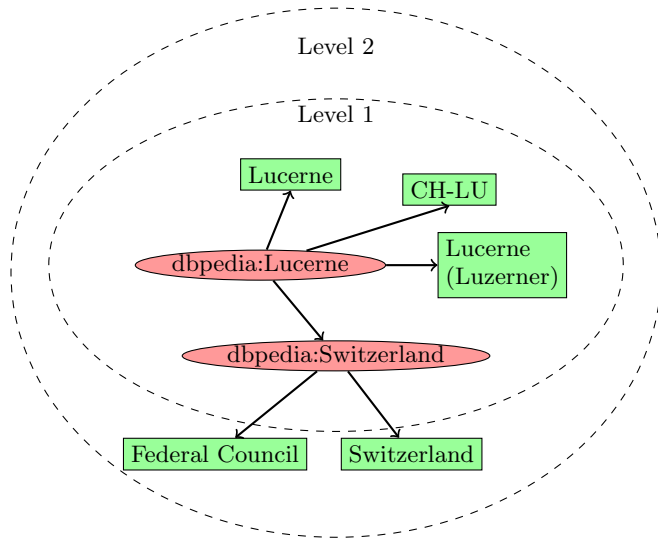
Figure 3: Creation of Virtual Documents by Levels.
