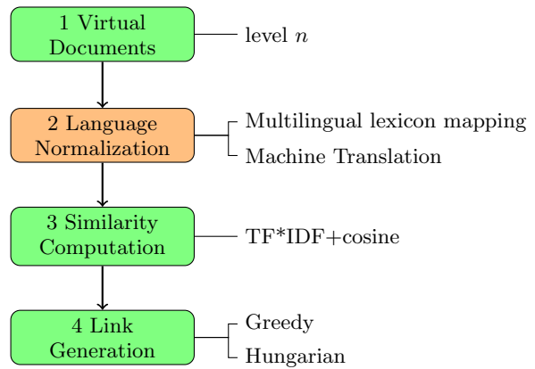
Figure 1: Framework for Cross-lingual RDF Interlinking.
