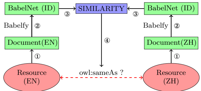
Figure 2: Interlinking Method Using Multilingual Lexicon. Multilingual terms are mapped to a common identifier. Similarity is computed between identifiers. Numbers correspond to the steps of the method.
