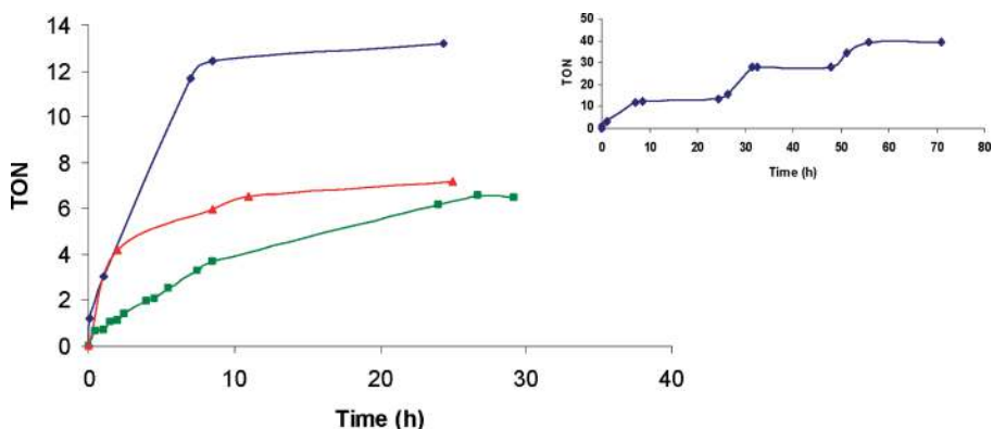
Figure 2. Catalytic oxidation of methylphenylsulfide (600 mM) to the corresponding sulfoxide using 1 (◆), 2 (■), and 3 (▲) as the catalyst (1 mM) and \text{H}_2\text{O}_2 (15 equiv) as the oxidant in acetone. Inset: the reaction catalyzed by 1 is monitored through the addition of three portions of hydrogen peroxide (15 equiv each).
