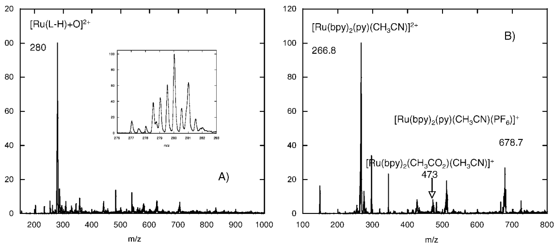
Figure 6. (A) ESI-MS spectra of 1 with \text{H}_2\text{O}_2 after 24 h reaction; inset: fragment at m/z 280. See Supporting Information for comparison with theoretical spectrum. (B) ESI-MS spectrum of 3 with \text{PhI}(\text{OAc})_2 after 80 h reaction. The arrow indicates the fragment of the acetato adduct.
