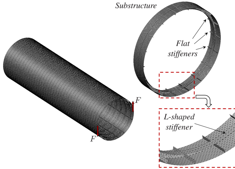
Figure 10: FE model of a stiffened cylindrical shell composed of 20 substructures.
