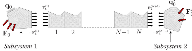
Figure 2: Periodic structure connected to two elastic subsystems.
