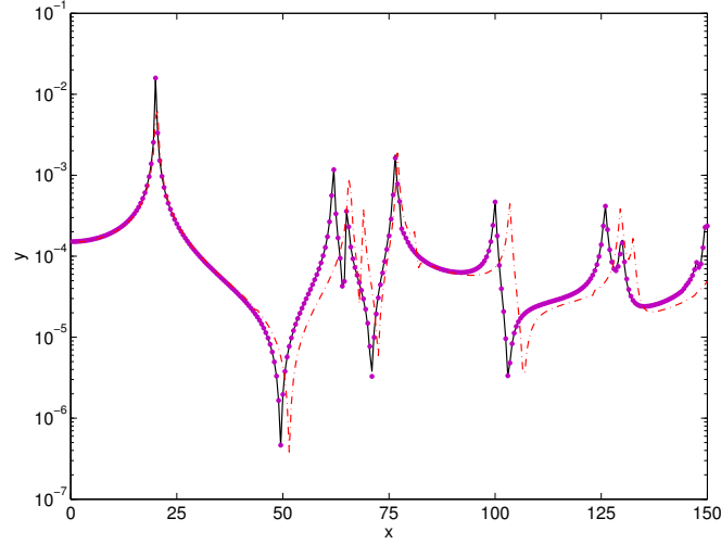
Figure 11: FRF of the stiffened cylindrical shell (fine mesh): FE solution (—) and WFE solution when the central periodic structure is modeled by means of m = 125 wave modes ( \bullet \bullet \bullet ); (coarse mesh): FE solution ( - \cdot - ).
