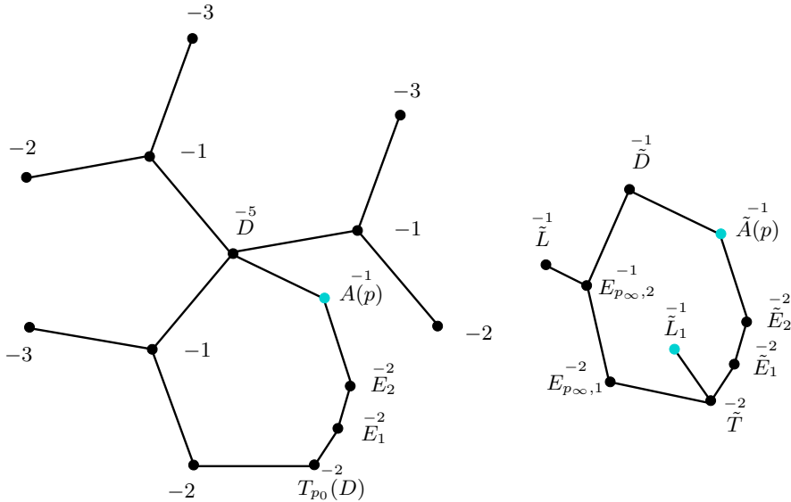
FIGURE 5.7. Dual graphs of the total transforms of B \cup A(p) and \tilde{B} \cup \tilde{A}(p) \cup \tilde{L}_1 in a minimal log-resolution of the pairs (V, B) and (\tilde{V}, \tilde{B}) respectively for (\mu, \nu) = (3, 1) .
