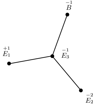
FIGURE 2.3. Dual graph of the proper transform of \tau^{-1}(B) by \theta_1 .
