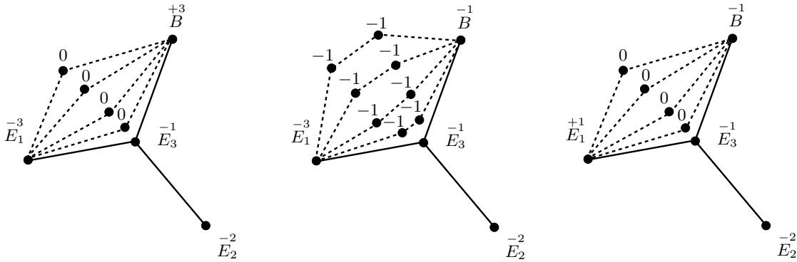
FIGURE 2.4. Elementary transformations.
