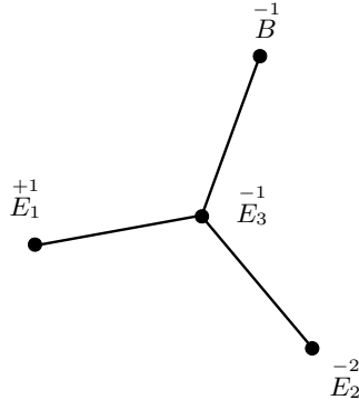
FIGURE 2.3. Dual graph of the proper transform of \tau^{-1}(B) by \theta_1 .
