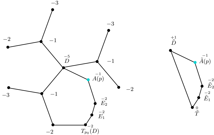
FIGURE 5.7. Dual graphs of the total transforms of B \cup A(p) and \tilde{B} \cup \tilde{A}(p) in a log-resolution of the pairs (V, B) and (\tilde{V}, \tilde{B}) respectively for (\mu, \nu) = (3, 1) .
