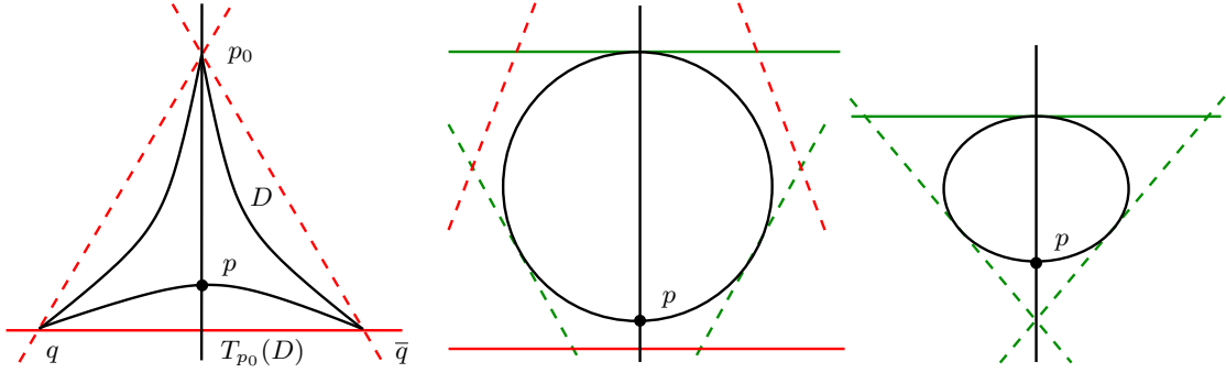
FIGURE 5.6. Behavior of the tricupidal quartic under the standard Cremona transformation.
