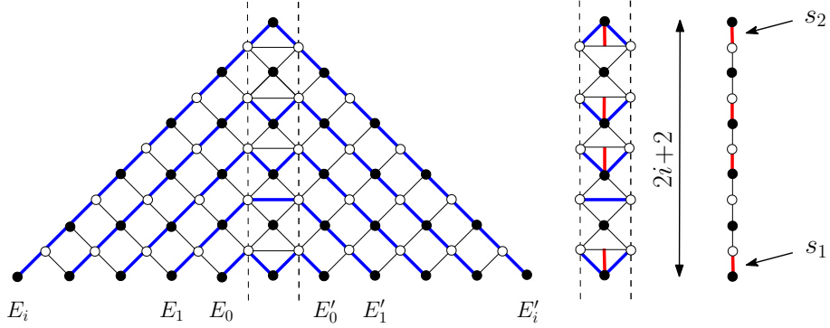
FIGURE 14. Mutually avoiding paths on the graph of Figure 13, from E_0, E_1, \dots, E_i to E'_0, E'_1, \dots, E'_i . The only freedom comes from the central column (between abscissas -1 and 1 ). The path configurations in this column are in one-to-one correspondence with hard dimers on a bicolored segment of length 2i+2 .
