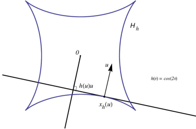
Figure 2. A plane hedgehog with a C^2 -support function
