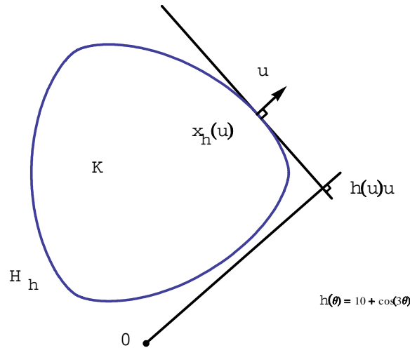
Figure 1. Hedgehogs as envelopes parametrized by their Gauss map
