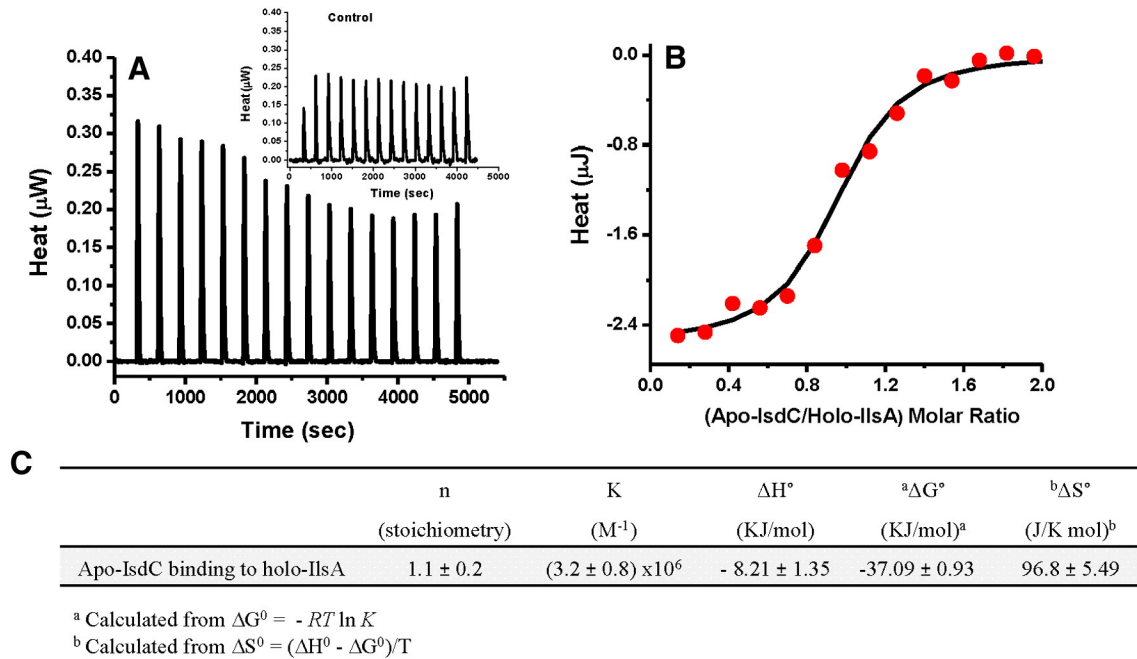
Fig. 7. Isothermal titration calorimetry (ITC) of apo-IsdC binding to holo-IsIA. Holo-IsIA (15 µM) is titrated with 3 µl injections of apo-IsdC (109 µM) in 50 mM Tris/HCl buffer, 150 mM NaCl, 1 mM EDTA and 1 mM DTT, pH 7.0 and 25 °C. (A) ITC raw data. (B) Plot of the integrated heat versus the molar ratio of apo-IsdC to holo-IsIA and best fit to the data. (C) ITC thermodynamic parameters for apo-IsdC binding to holo-IsIA. At least three independent determinations were made and the standard deviation of fitted parameters is provided. Additions of apo-IsIA to apo-IsdC yielded heats similar to the control experiment suggesting that heme is required for the association of holo-IsIA to apo-IsdC.
