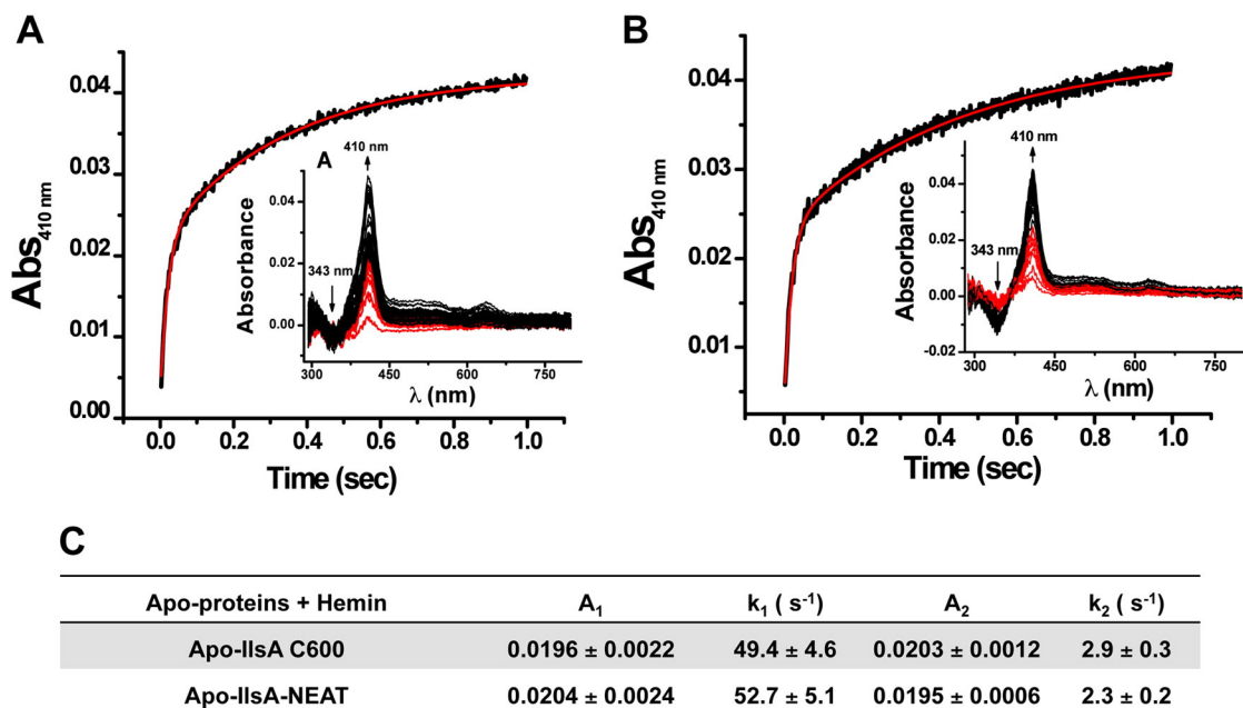
Fig. 4. Absorbance time curves at 410 nm for hemin association with apo-IlsA and apo-NEAT IlsA . (A) 15 \mu M apo-IlsA or (B) apo-NEAT IlsA and 10 \mu M hemin; both protein solutions were in 50 mM Tris, 150 mM NaCl, pH 7.4 and 25 °C. The red curves are the best fit to the experimental data in black using two exponential equations. The insets are the family of stopped-flow UV-Vis spectra gathered every 2.5 ms for the first 40 ms (red) of the reaction and every 50 ms (black) thereafter. (C) First order rate constants ( k_1 and k_2 ) and the corresponding absorbance values ( A_1 and A_2 ); both proteins are produced in E. coli C600 and presumed to be heme free.
