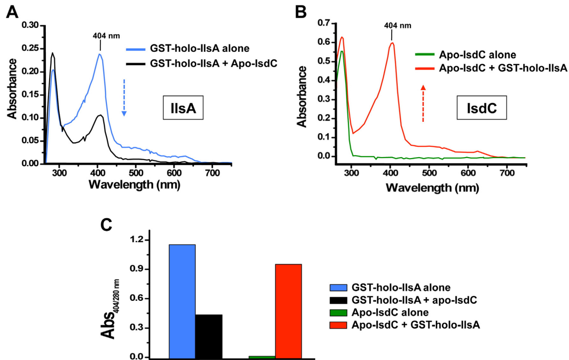
Fig. 8. Hemin transfer from holo-IsIA to apo-IsdC. GST-apo-IsIA (10 µM) was loaded onto a glutathione–sepharose gel, charged by heme and then incubated with apo-IsdC (50 µM) for 30 min at 25 °C. Supernatant and sediment were separated by centrifugation and GST-IsIA was collected by elution with reduced glutathione. The fractions containing (A) IsIA and (B) IsdC were analyzed by UV–Vis and (C) the heme content was quantified using the 404/280 ratio.
