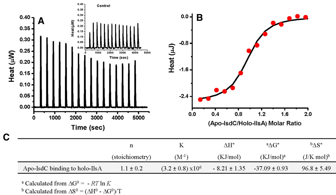
Fig. 7. Isothermal titration calorimetry (ITC) of apo-IsdC binding to holo-IsIA. Holo-IsIA (15 μM) is titrated with 3 μl injections of apo-IsdC (109 μM) in 50 mM Tris/HCl buffer, 150 mM NaCl, 1 mM EDTA and 1 mM DTT, pH 7.0 and 25 °C. (A) ITC raw data. (B) Plot of the integrated heat versus the molar ratio of apo-IsdC to holo-IsIA and best fit to the data. (C) ITC thermodynamic parameters for apo-IsdC binding to holo-IsIA. At least three independent determinations were made and the standard deviation of fitted parameters is provided. Additions of apo-IsIA to apo-IsdC yielded heats similar to the control experiment suggesting that heme is required for the association of holo-IsIA to apo-IsdC.
