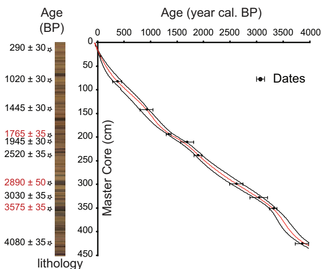
Figure 3. Lithology of MC LL081 and age–depth model based on radiocarbon calibrated ages (AMS; see Table 1) from LL081 and LL082 (in red).
